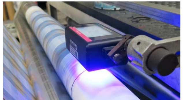
CCD Image Sensor DC-01 is used on Line Position Control
